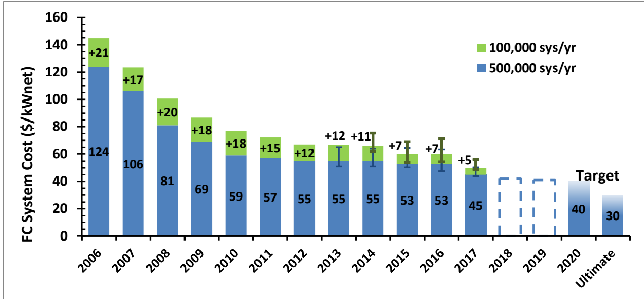
Figure 1. Modeled cost of an 80-kW net PEM fuel cell system based on projection to high-volume manufacturing (100,000 and 500,000 units/year). Reported values from 2012 and earlier were adjusted to account for higher platinum price, realigned compressor and expander efficiencies, and the Q/ΔT requirement introduced in 2013 (see 2013 cost record) [7]. Error bars represent the 90% confidence interval from a stochastic uncertainty analysis and reflect manufacturing uncertainty in the modeled system.
