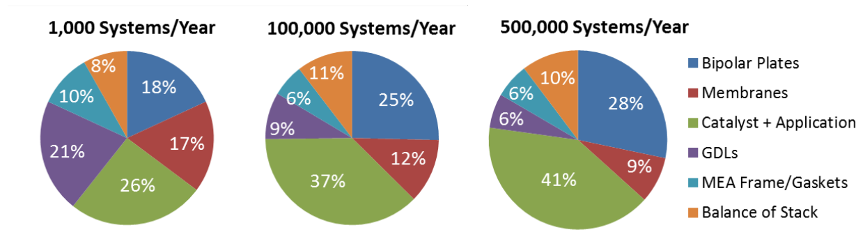
Figure 5. Breakdown of the 2017 projected fuel cell stack cost at 1,000, 100,000, and 500,000 systems per year.
