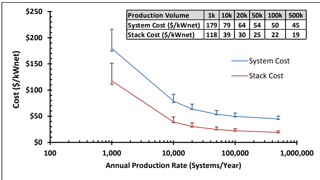
Figure 2. Projected cost of 2017 80-kW net transportation fuel cell stacks and systems at 1,000, 10,000, 20,000, 50,000, 100,000, and 500,000 units/year.
