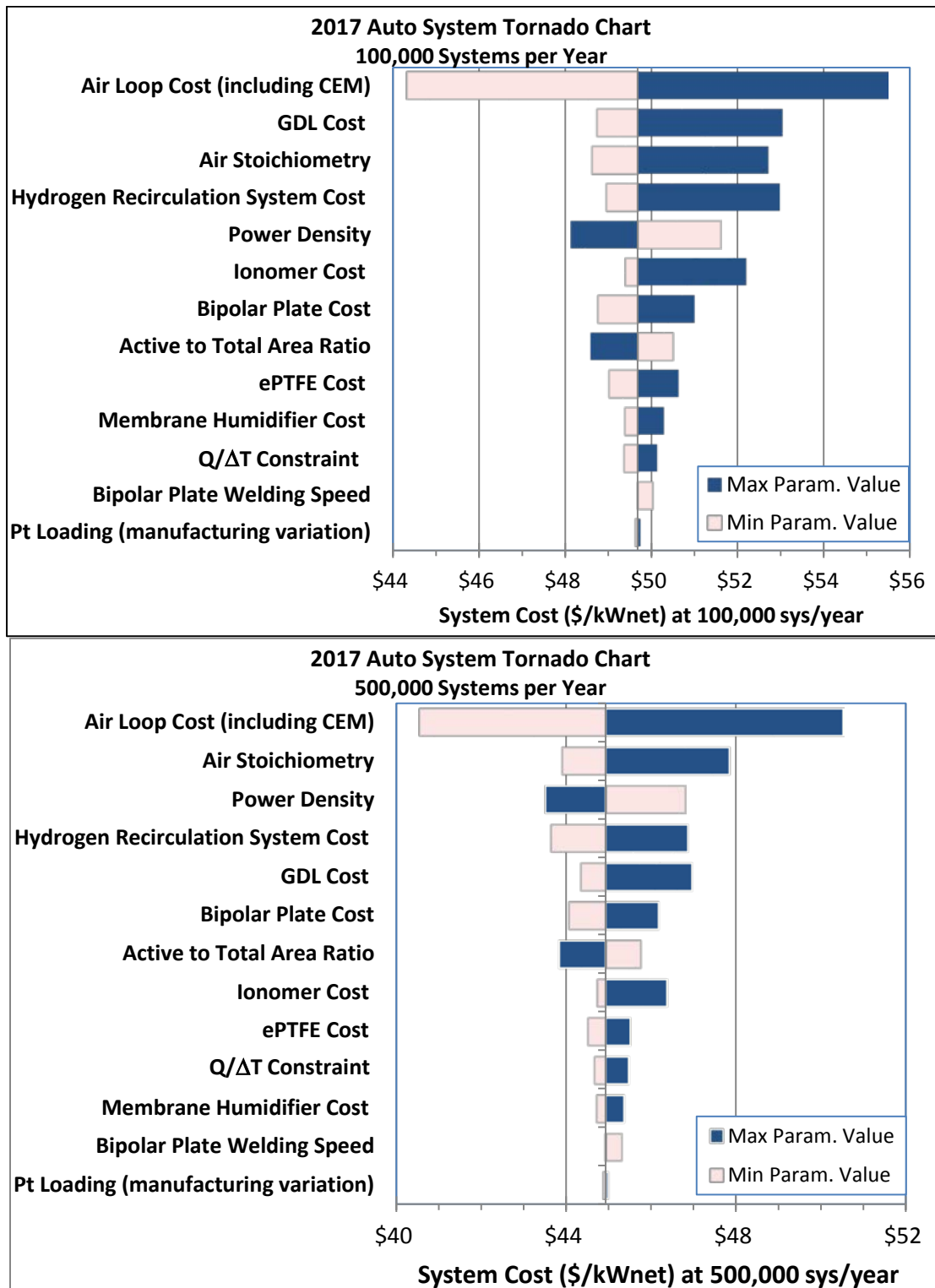
Figure 3. Tornado chart of single variable sensitivity analysis of system cost at 100,000 systems per year (top graph) and 500,000 systems per year (bottom graph). “CEM” refers to “compressor expander motor”.
