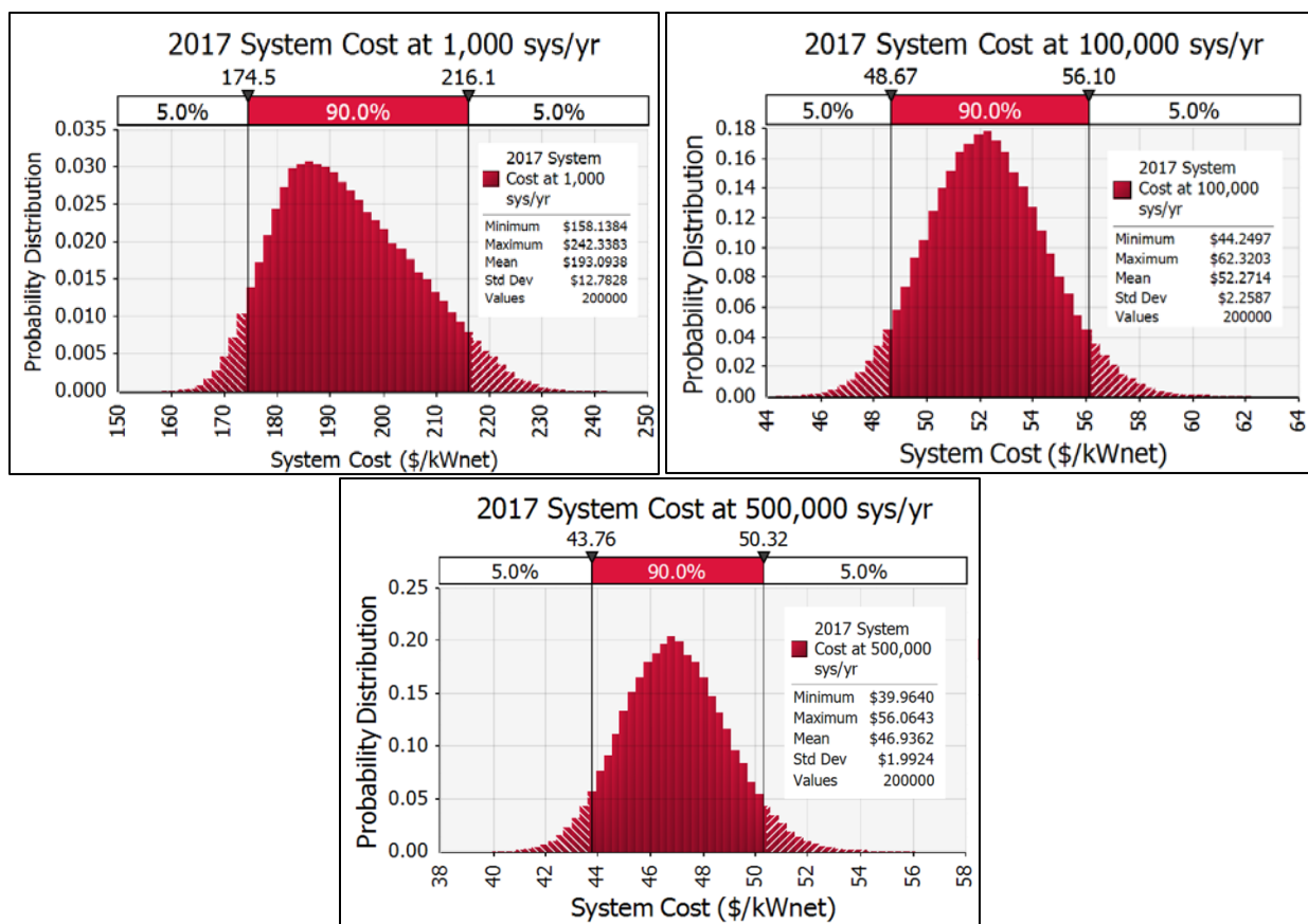
Figure 4. Monte Carlo analyses of system cost probability at 1,000, 100,000, and 500,000 systems per year.
